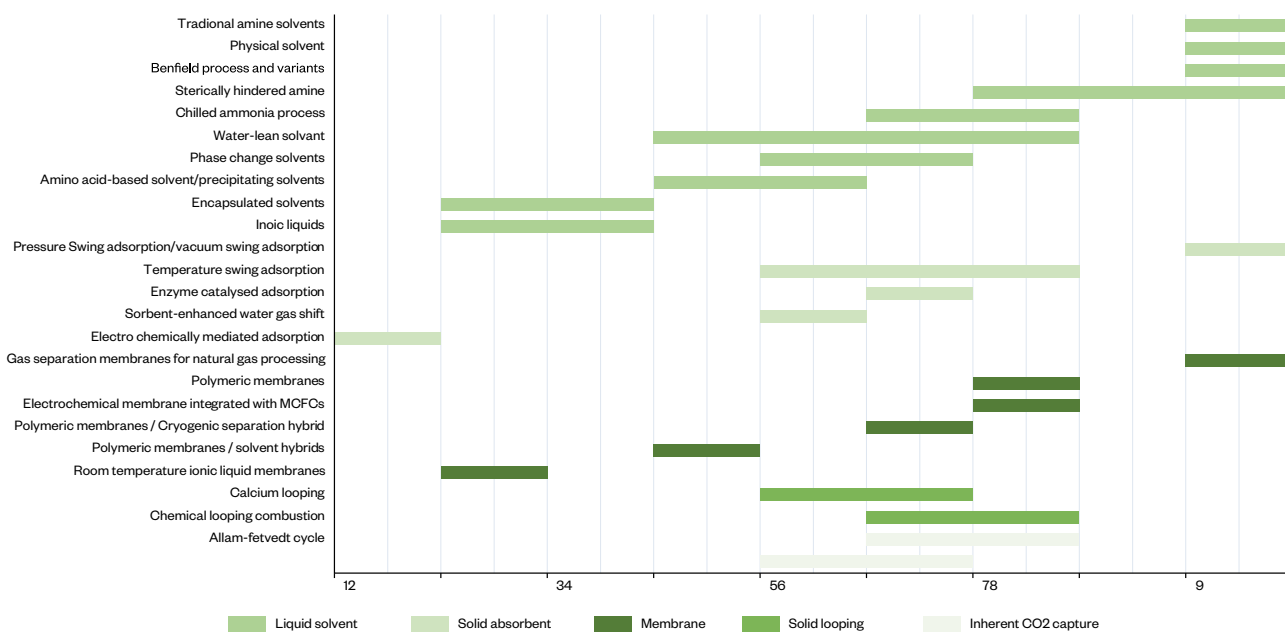
Figure 9: TRLs for CO 2 point source capture solutions
