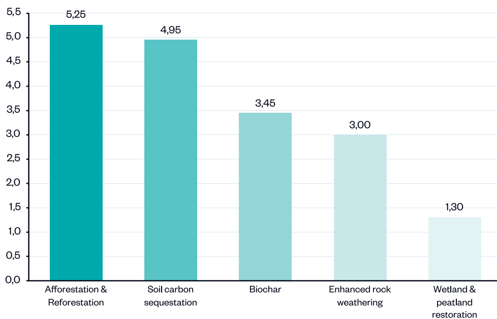
Figure 45: Global reduction potential of NbSs in 2050
